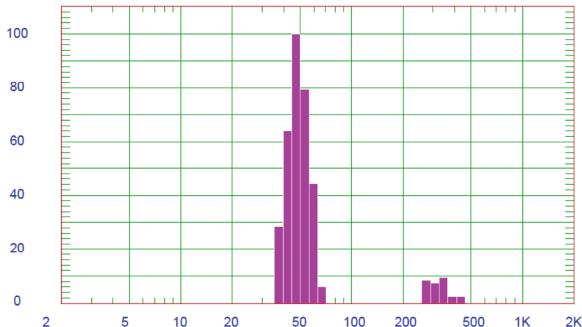
Fig. 3. The size distribution of hematite nanoparticles
