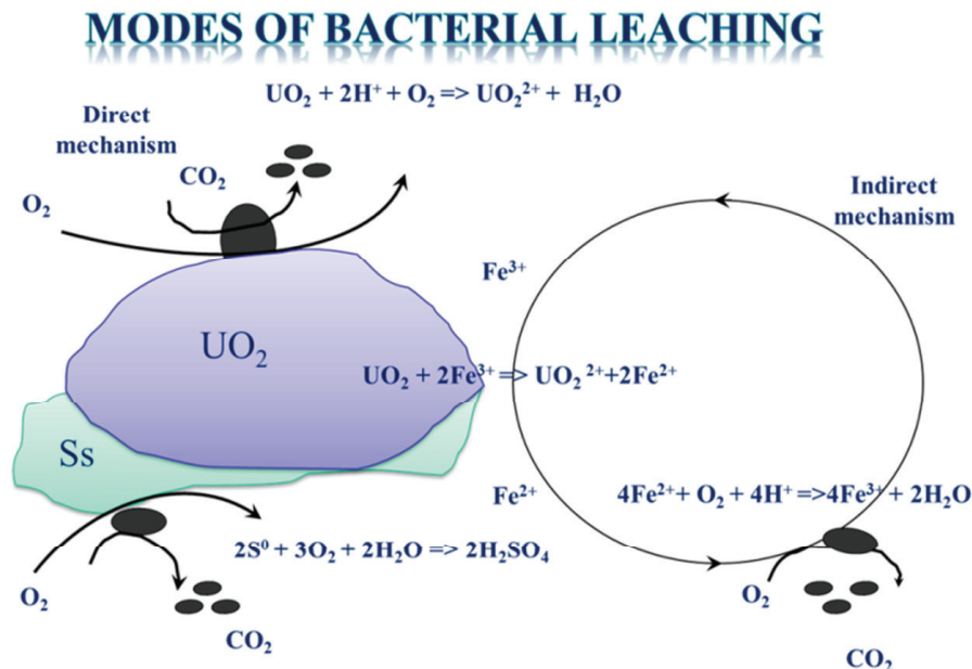
Fig. 1. Direct and indirect uranium bacterial leaching.
