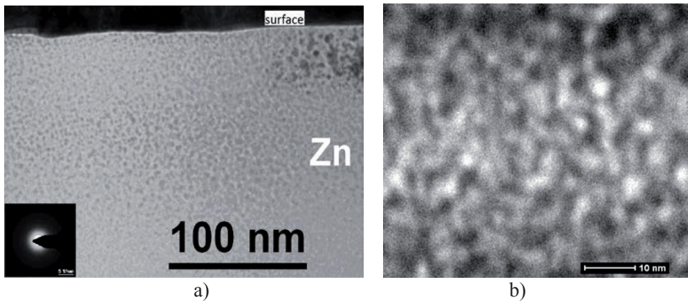
Figure 4: TEM survey image (a) and STEM image (b) for annealed sample of Zn NPs layer.
