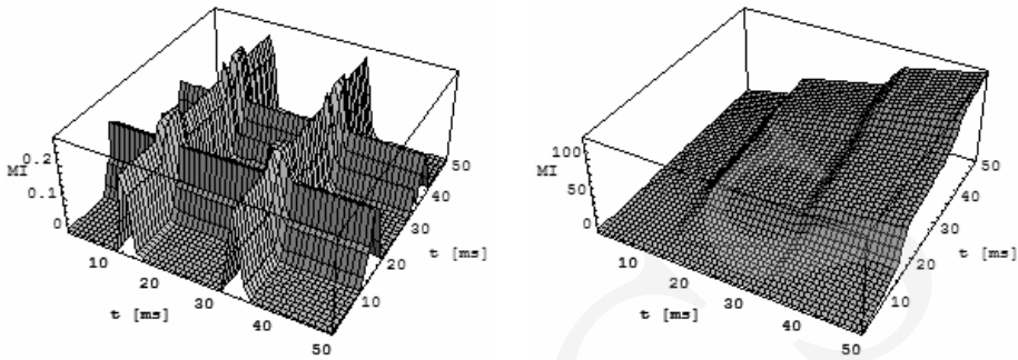
Fig. 6. Individual MI (left panel) and global MI (right panel) between two readout devices for the vertical pattern (see. Fig 3d). 3D MI maps were generated for the first 50 ms of simulation.
