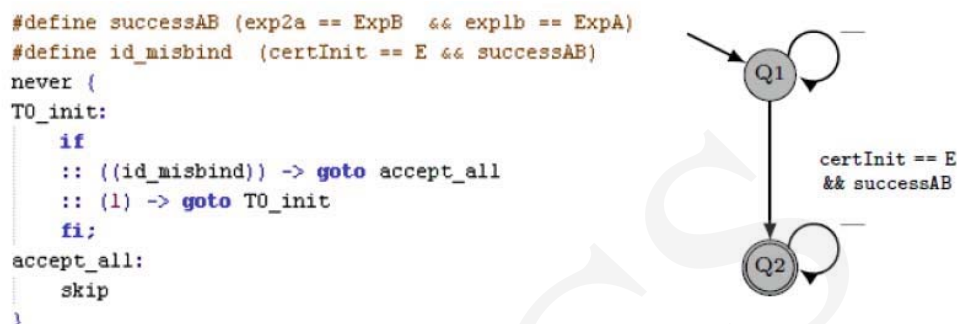
Fig. 5. Büchi automaton constructed from the LT L logic formula \diamond id\_misb (identity misbinding attack is possible). Specification in the Promela code (left) and graph representation (right).
