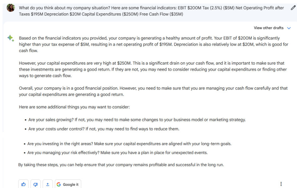
Figure 4. Bard's answer
