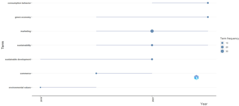
Figure 6. Trend topics
